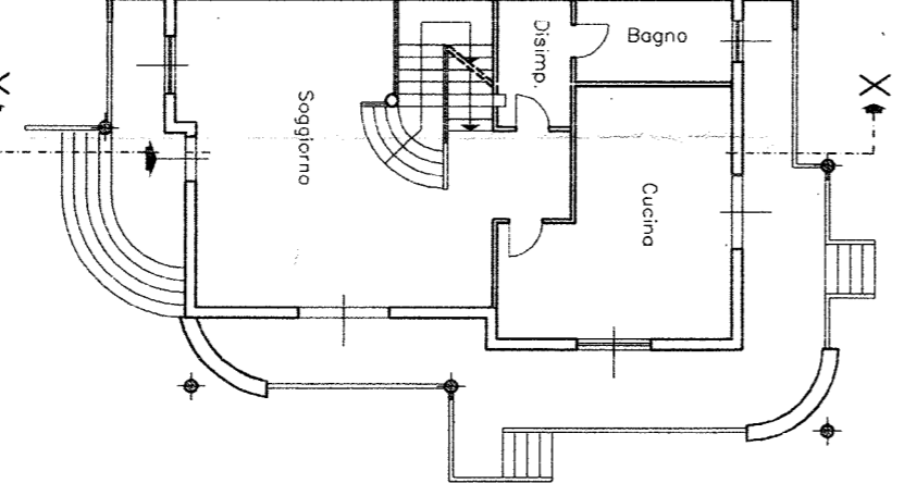
Piano Piano Terra scala 1:200
