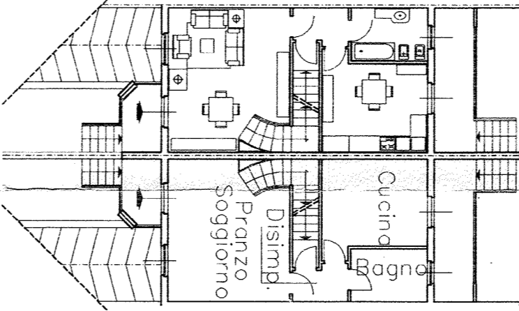
Piano Piano Terra scala 1:200
